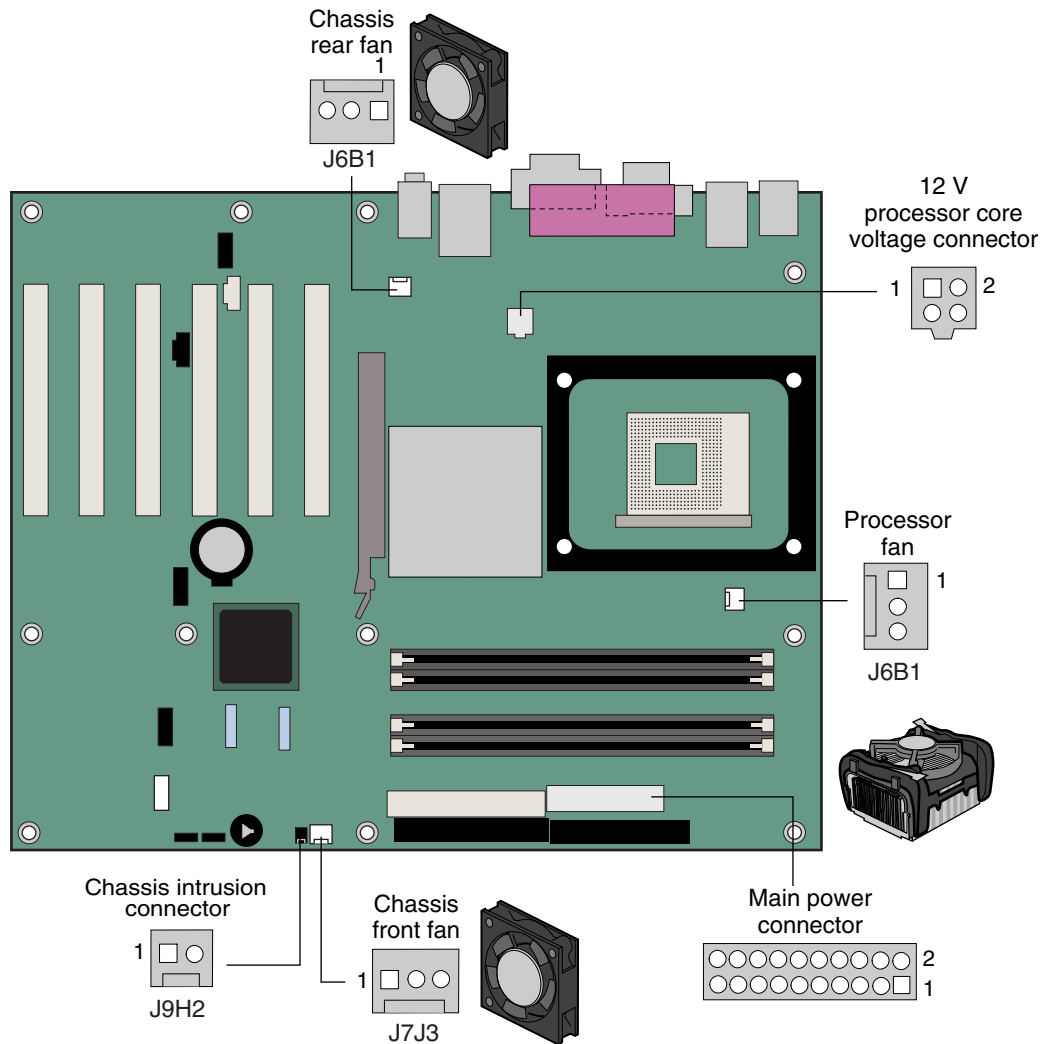
Figure 15. Location of Hardware Control Headers and Power Connectors
